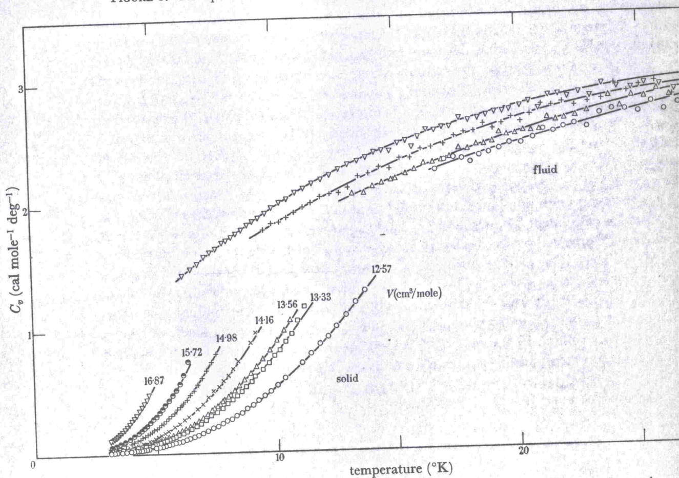
FIGURE 6. The specific heat at constant volume of solid and fluid 3 He at various volumes.
