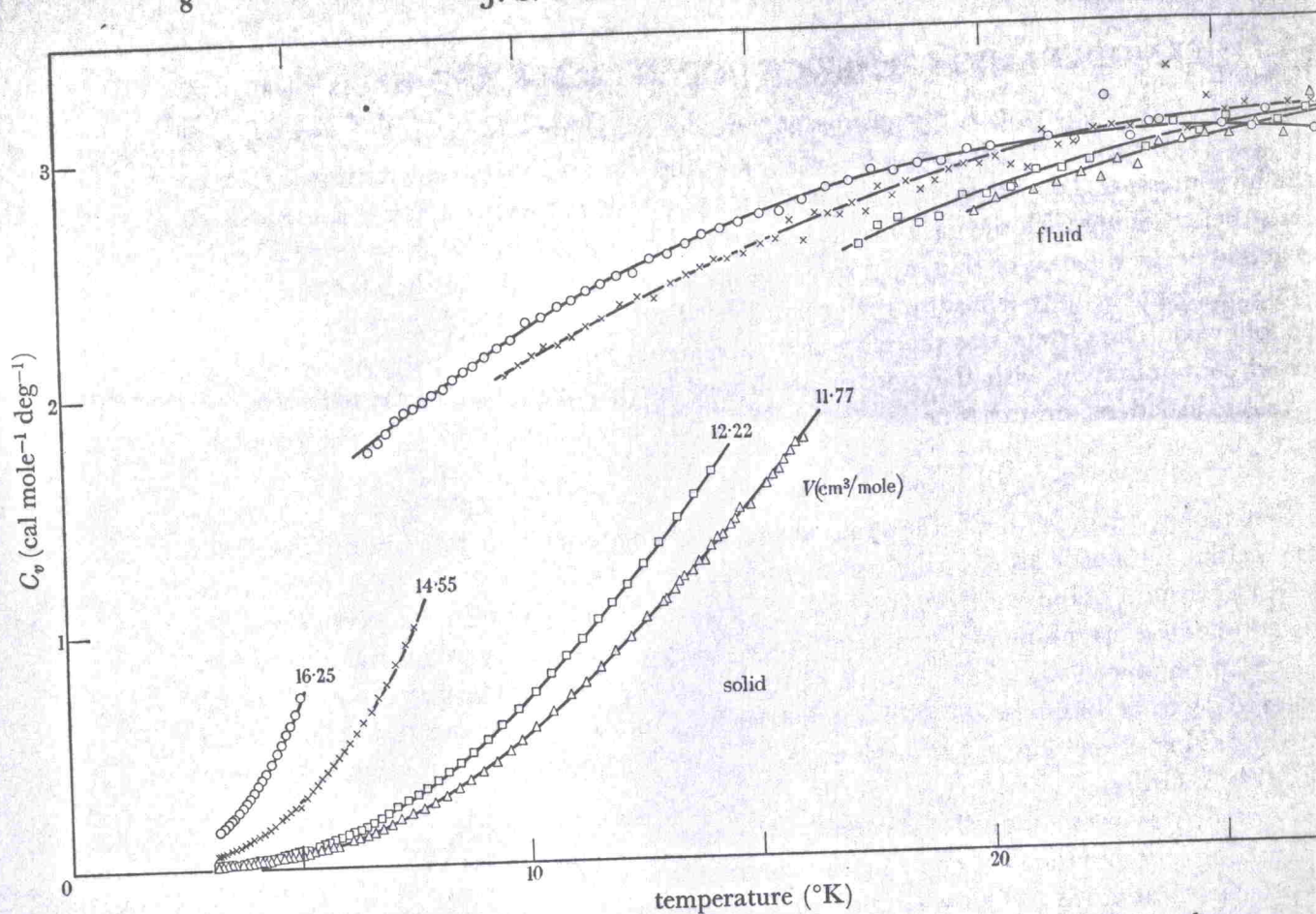
FIGURE 5. The specific heat at constant volume of solid and fluid 4 He at various volumes.
